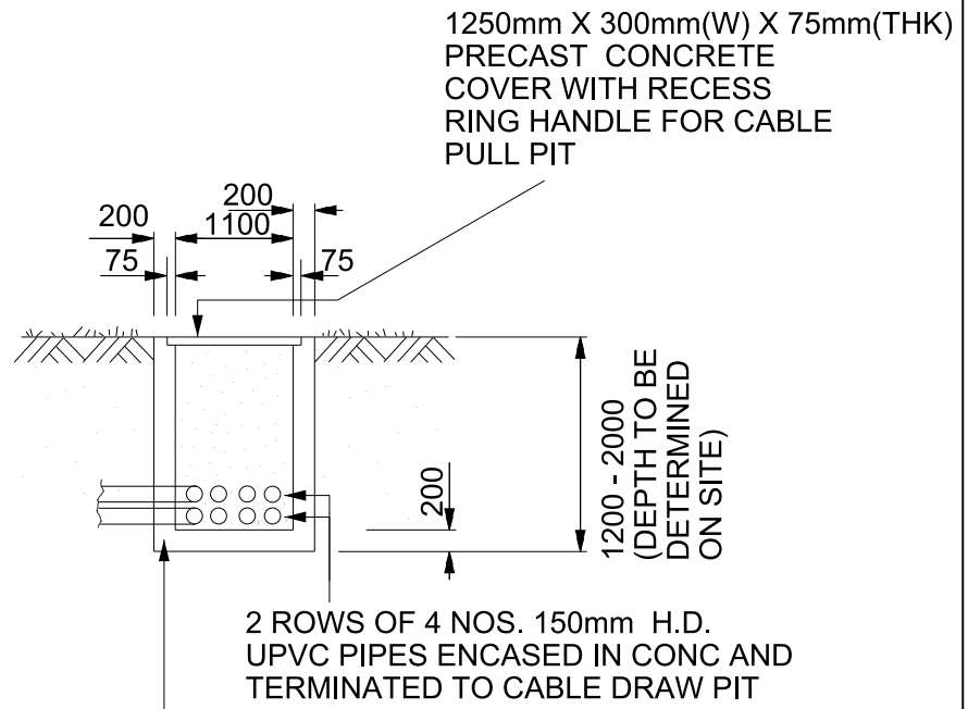
DETAIL OF EXPOSED CABLE DRAW PIT
