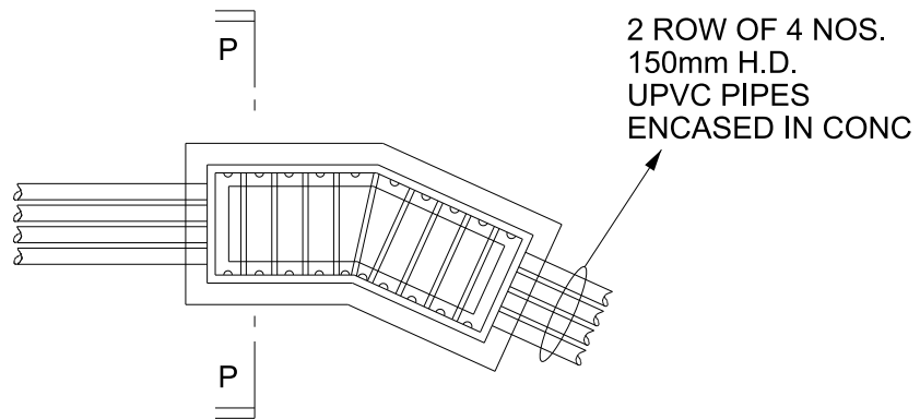
DETAIL OF EXPOSED CABLE DRAW PIT
